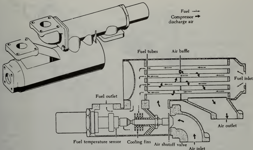
FIGURE 3-55. Fuel heater.
